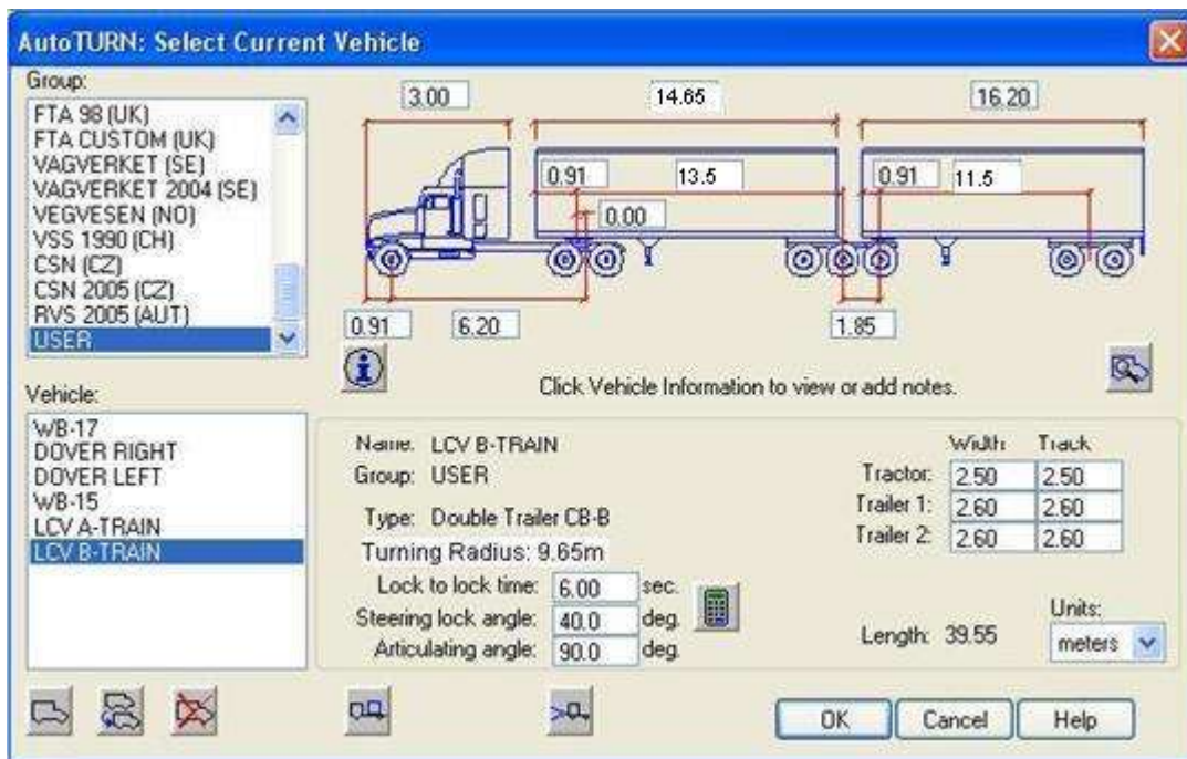
B-Train
